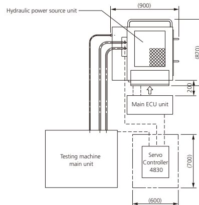
Example Layout for AF-20 Hydraulic Power Supply Unit
